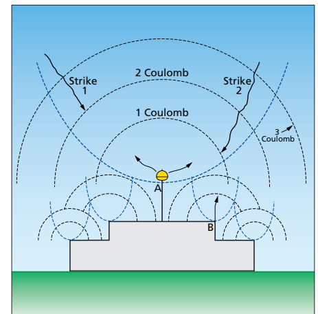
The Collection Volume Method defines the lightning “capture volume” of potential strike points on a structure. This method is used in conjunction with the ERITECH® SYSTEM 3000 lightning protection system but is equally applicable for the placement of conventional terminals.
